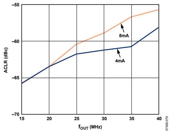
Figure 47. AD9117 2-Carrier W-CDMA First Adjacent Channel ACLR 1.8 V
