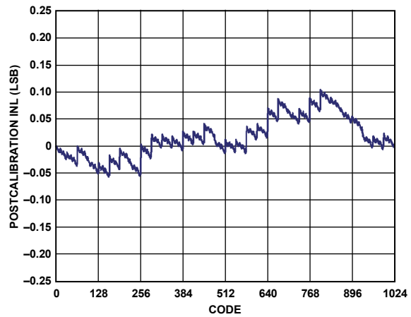
Figure 23. AD9115 Postcalibration INL at 1.8 V, 8 mA
