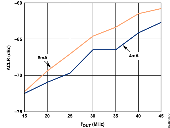
Figure 41. AD9117 1-Carrier W-CDMA First Adjacent Channel ACLR 1.8 V
