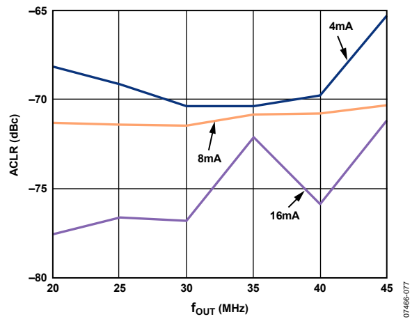
Figure 46. AD9117 1-Carrier W-CDMA Third Adjacent Channel ACLR 3.3 V
